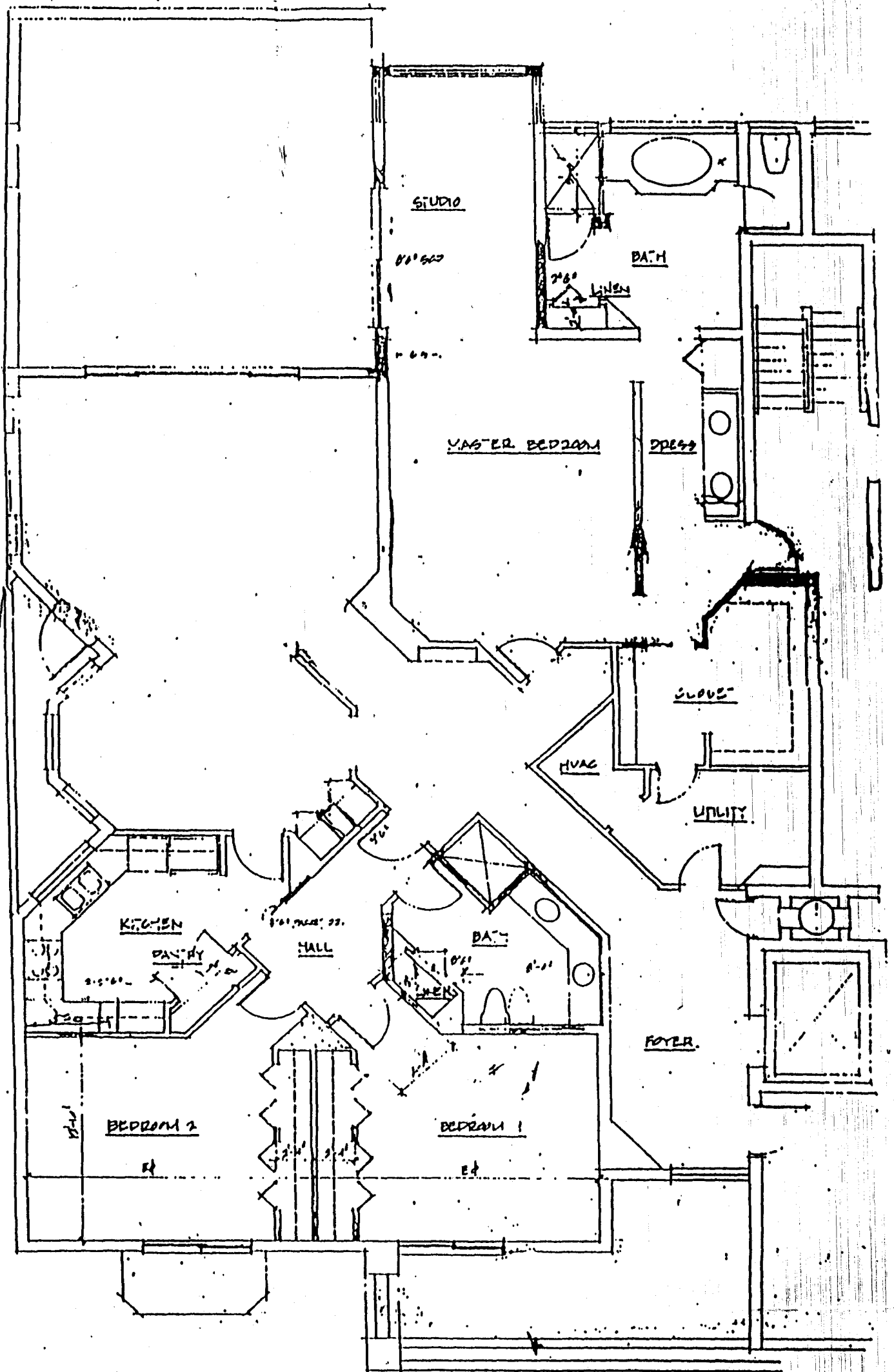
TYPICAL 3 BEDROOM UNIT ( 1st 2nd & 3rd FLOORS - NORTH SIDE ONLY
