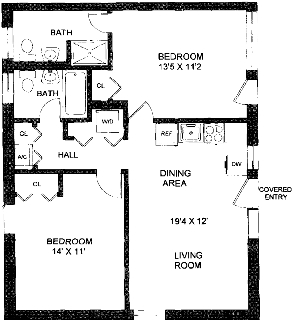
Two Bedroom, Two Bath Plan
