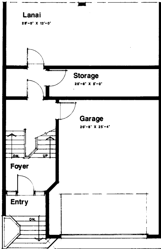
Typical Ground Floor Plan
