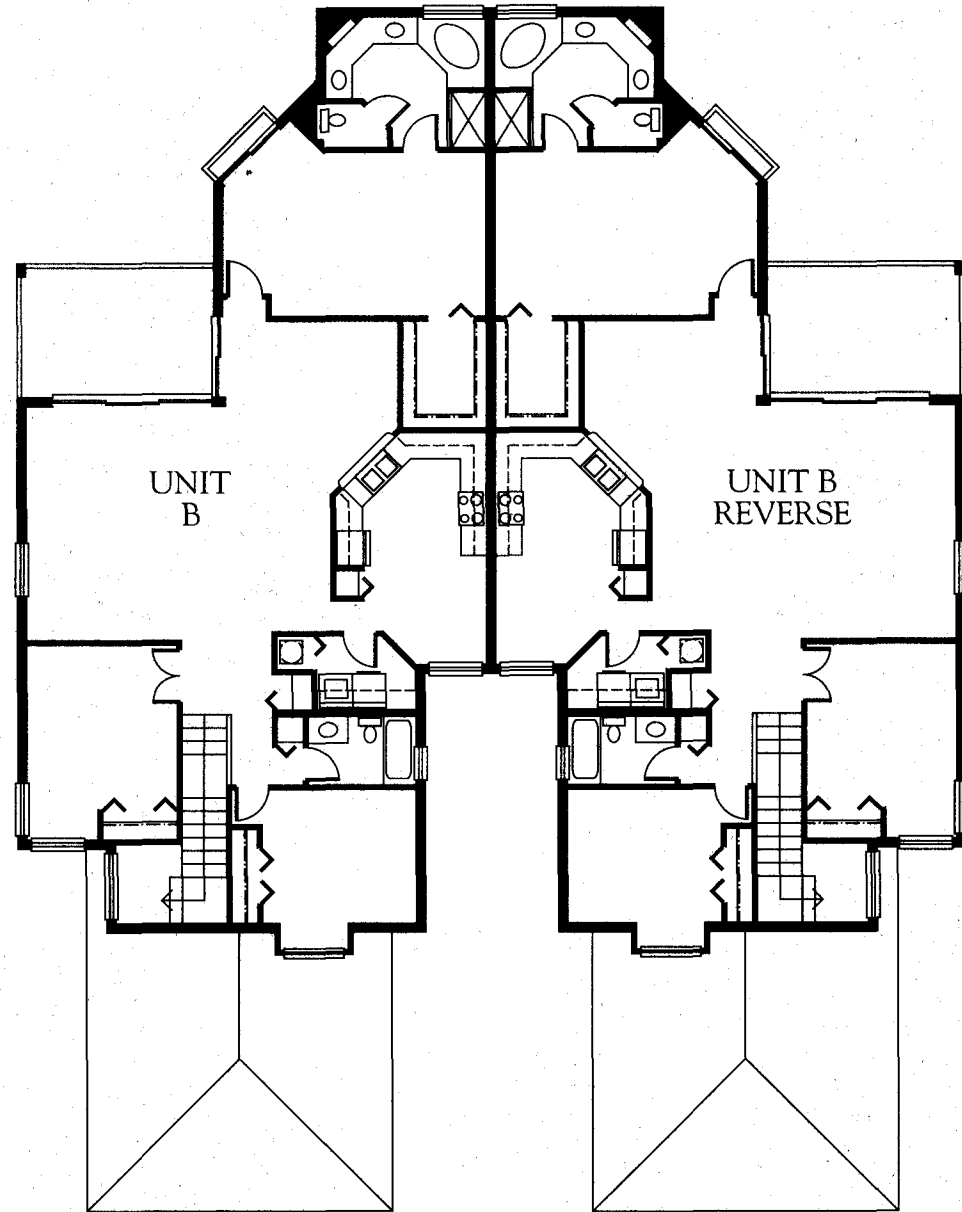
SECOND FLOOR BUILDING PLAN BUILDING TYPE I
