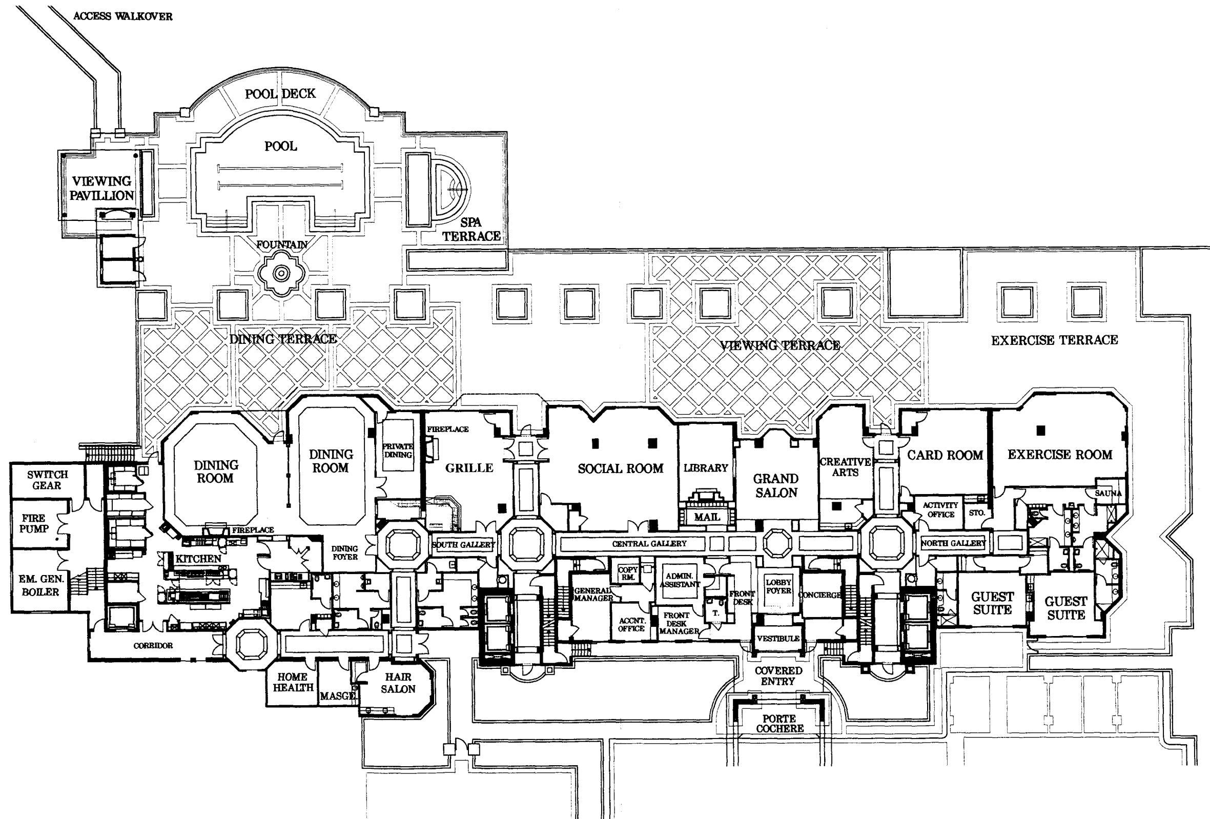
LOBBY LEVEL FLOOR PLAN
