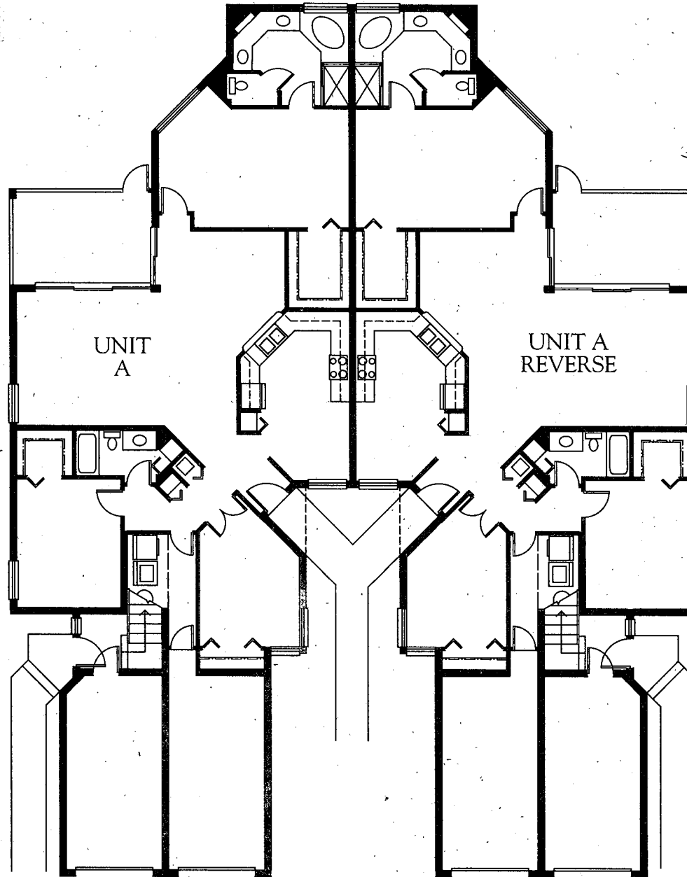
FIRST FLOOR BUILDING PLAN BUILDING TYPE I
