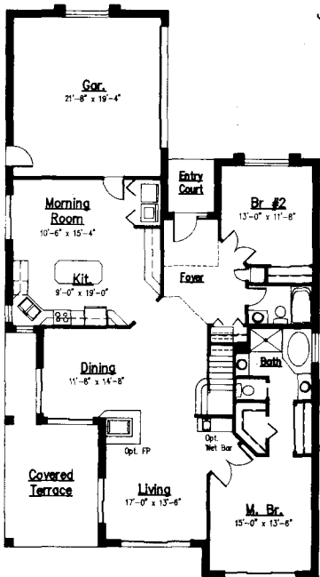
FLOOR PLAN E 2,377 SQ. FT.
